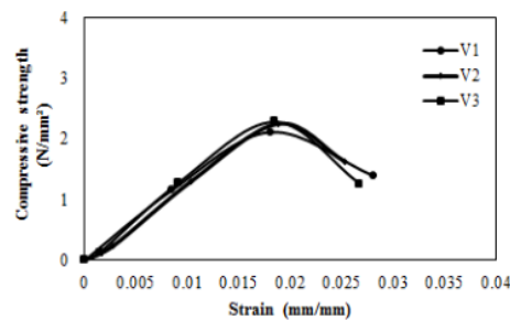
Fig 4. Stress-strain relationship of specimens immersed in \text{Na}_2\text{SO}_4 solution
