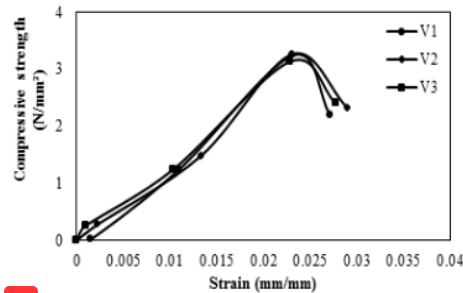
13 Fig 3. Stress-strain relationship of specimens immersed in the water
